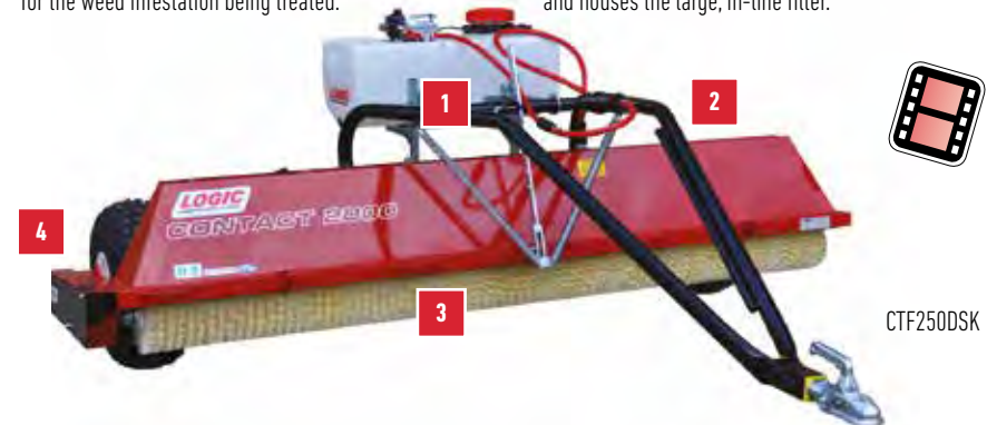
Height adjustment is spring-assisted to allow the machine to be quickly and easily set to the correct working height for the weed infestation being treated.
